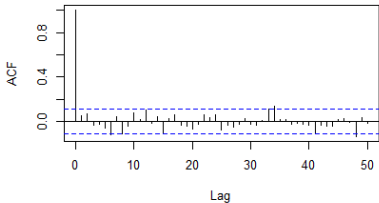
Daily change in Dow Jones index
