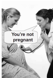
Type II error (false negative)
