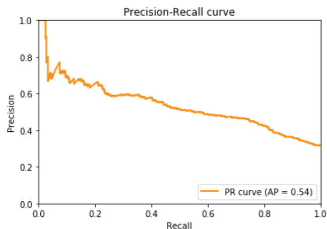
(b) PR-curve
