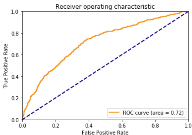
(a) ROC-curve
