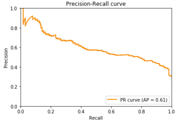
(b) PR-curve
