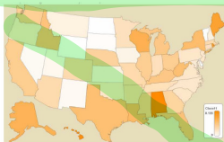
With PLSA
