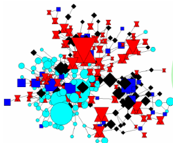
PLSA
