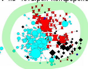
NetPLSA
