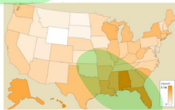
With NetPLSA
